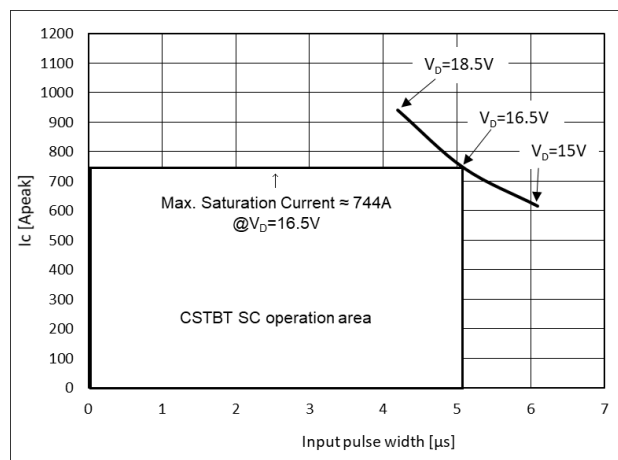
Fig.3-1-15 Typical SCSOA curve of PSS75NE1CT
