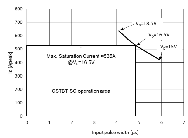
Fig.3-1-14 Typical SCSOA curve of PSS50NE1CT
