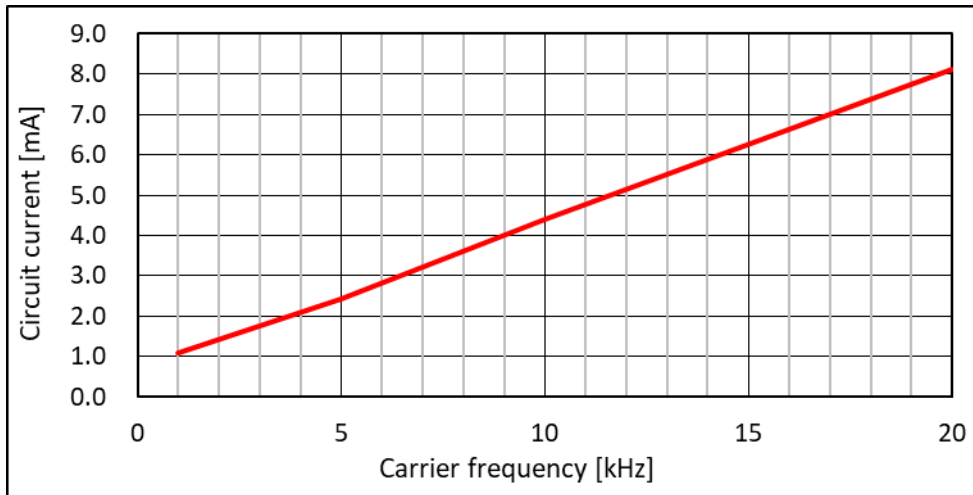
Fig. 4-2-2. I_{DB} vs. Carrier frequency for PSS75NE1CT
