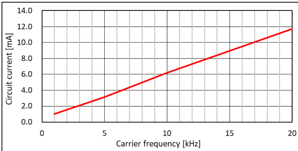
Fig. 4-2-3. I_{DB} vs. Carrier frequency for PSS100NE1CT
