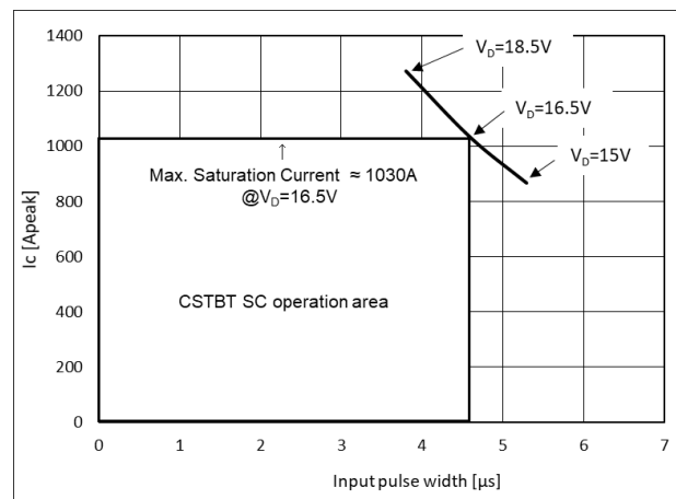
Fig.3-1-16 Typical SCSOA curve of PSS100NE1CT
