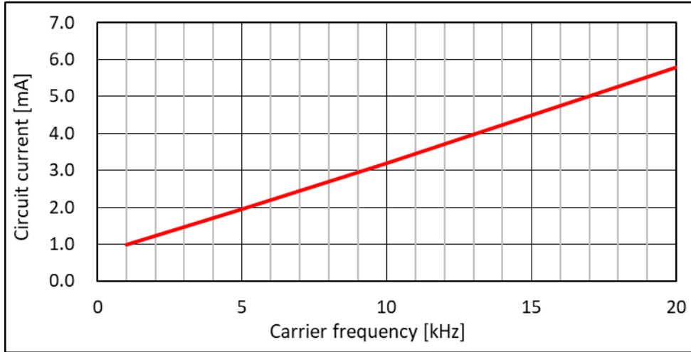
Fig. 4-2-1. I_{DB} vs. Carrier frequency for PSS50NE1CT
