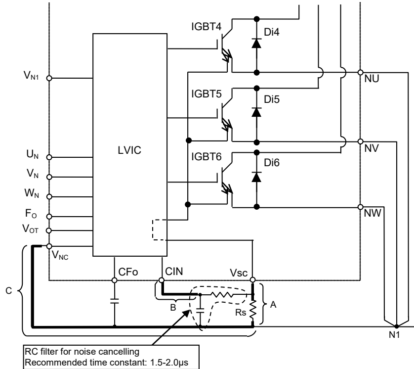
Fig.3-1-10 External protection circuit
